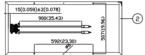
back side
