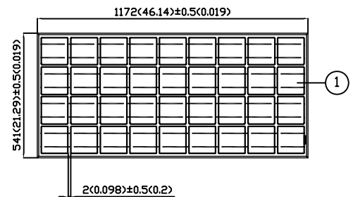
Front side
